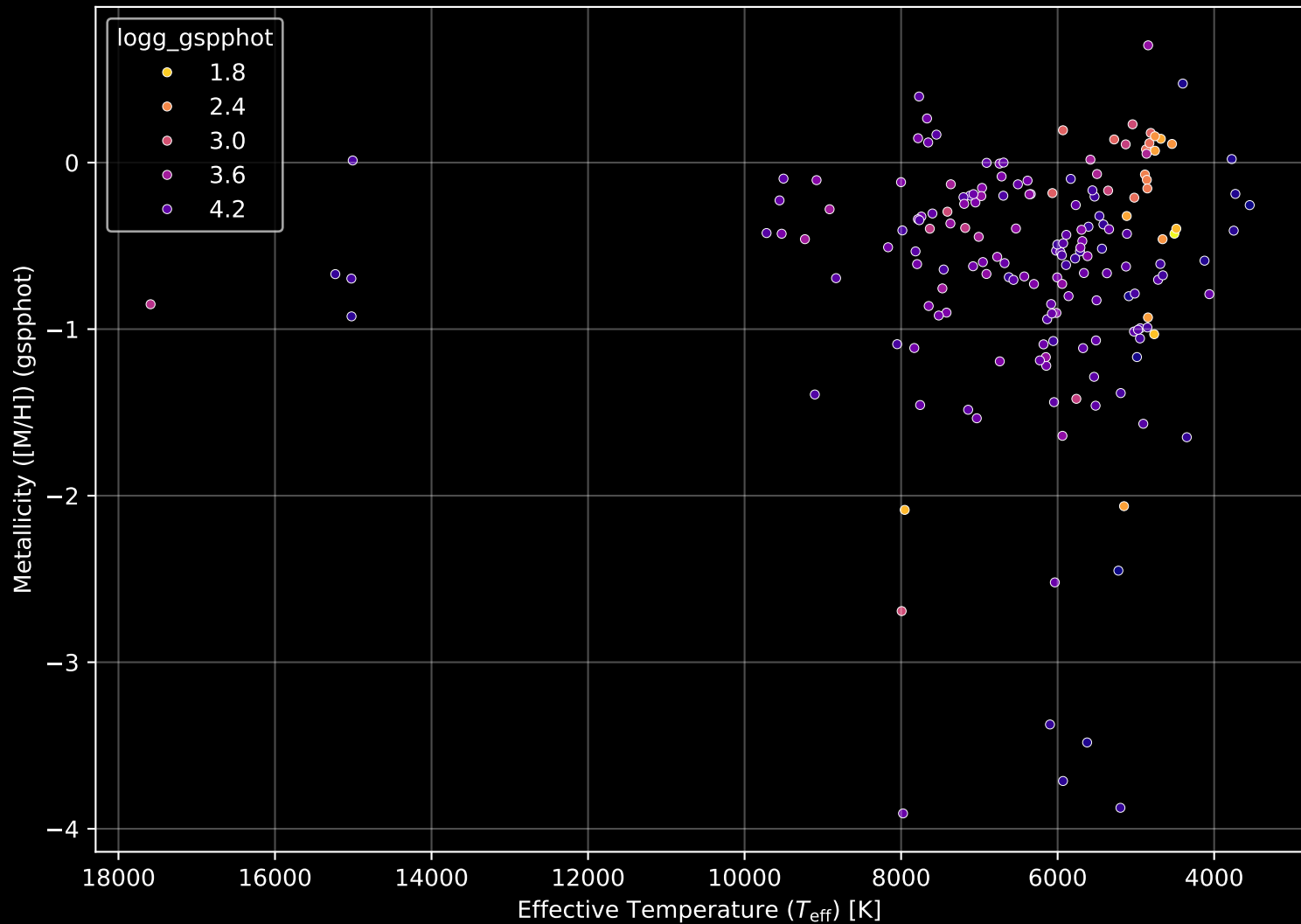
APOGEE DR17 Field: [K2_C11_003+05_btx] Stellar Population Parameters (n= 175)
