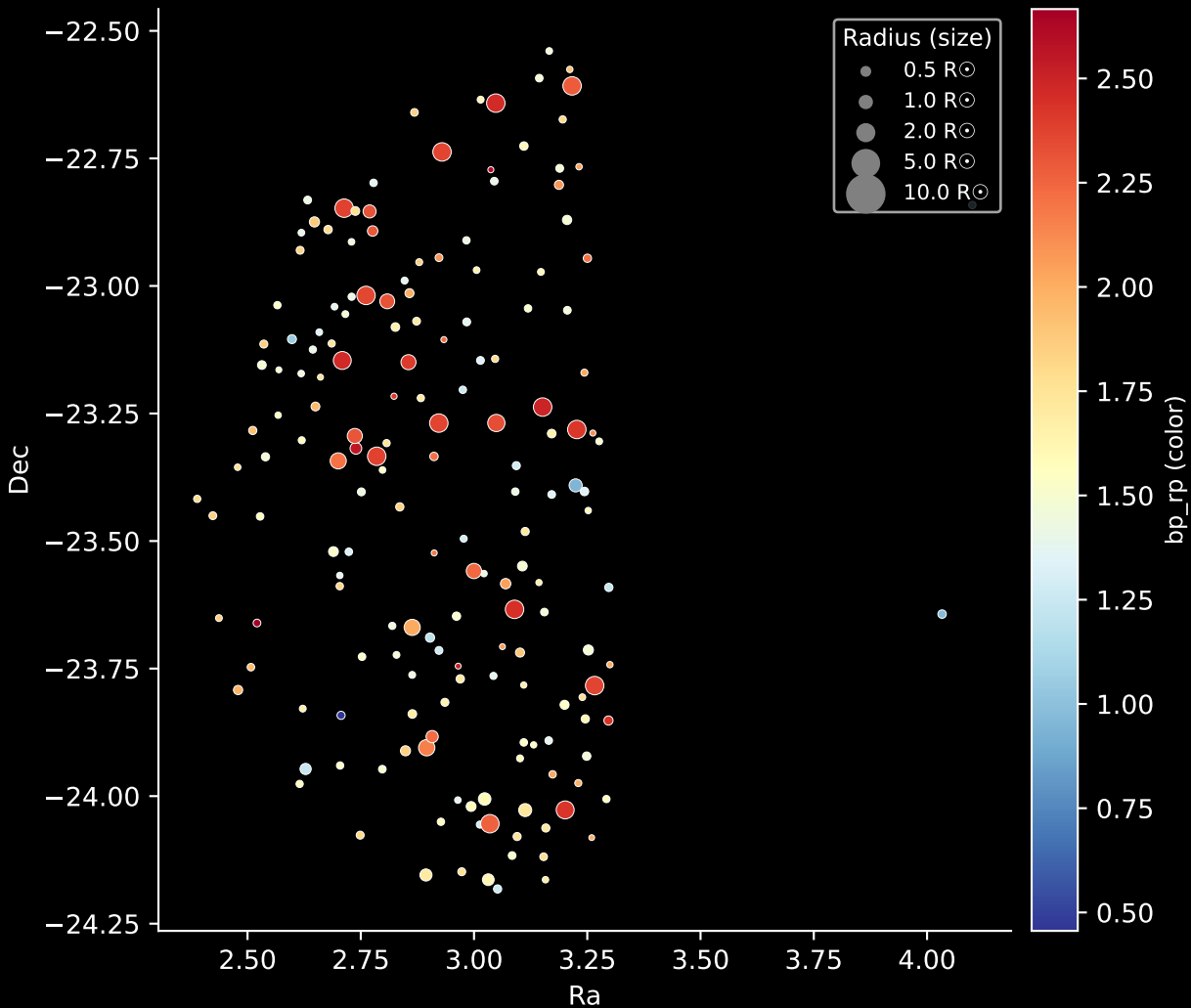
APOGEE DR17 Field: [K2_C11_003+05_btx] Stars: 175
