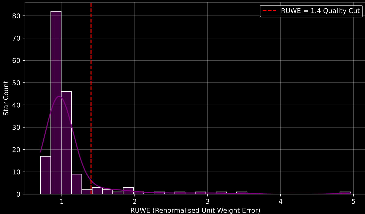
GAPOGEE DR17 Field [K2_C11_003+05_btx] RUWE Distribution (n= 172)
