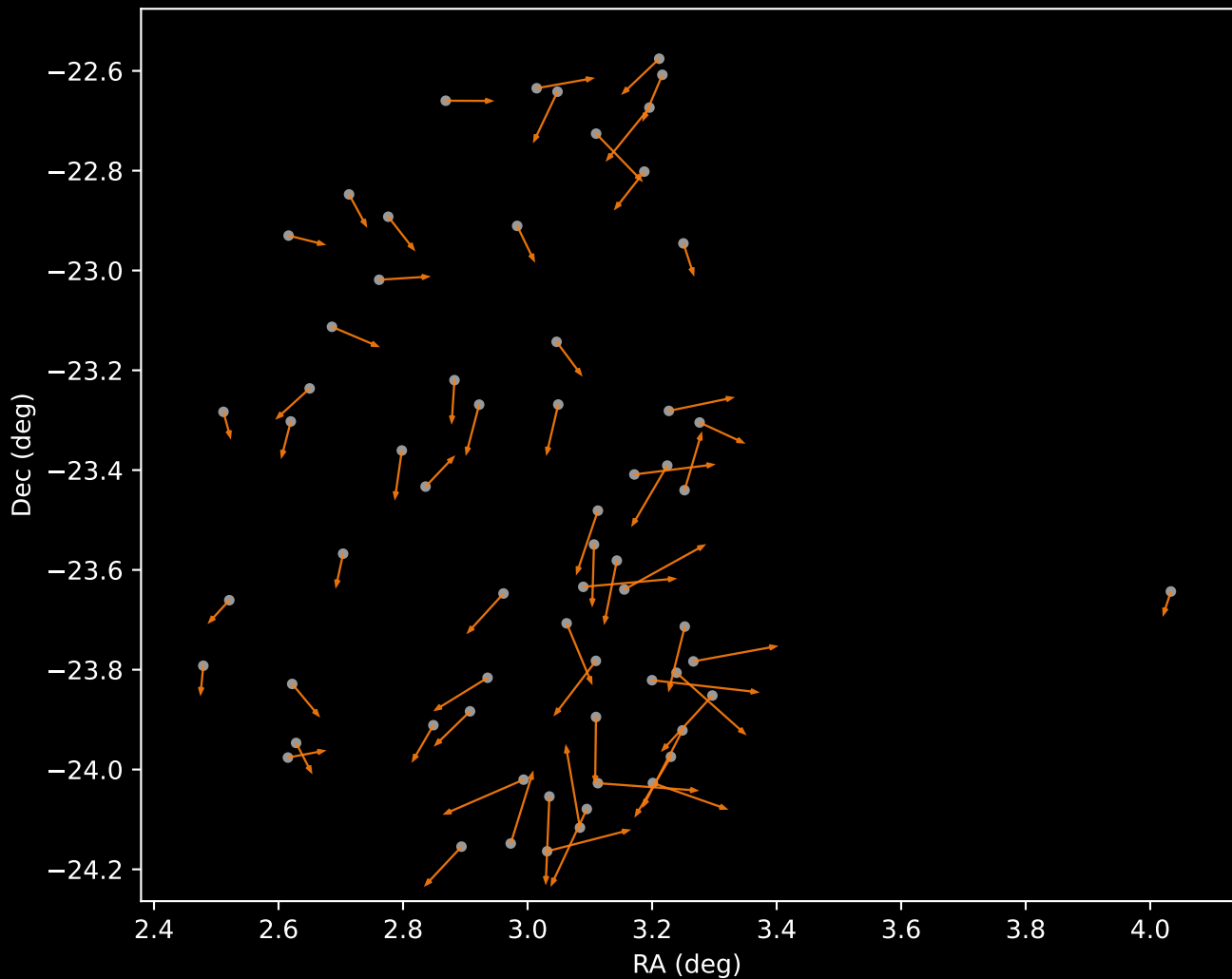
APOGEE DR17 Cluster 2 Proper Motion Vectors (n=64)
