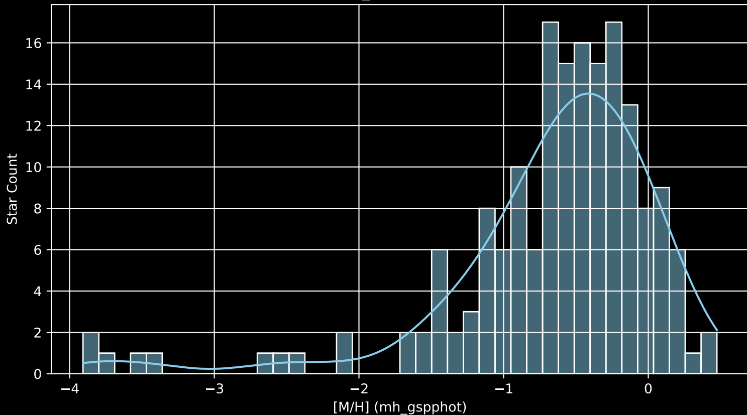
APOGEE DR17 Field: [K2_C11_003+05_btx [M/H] (mh_gspphot) (n= 174)
