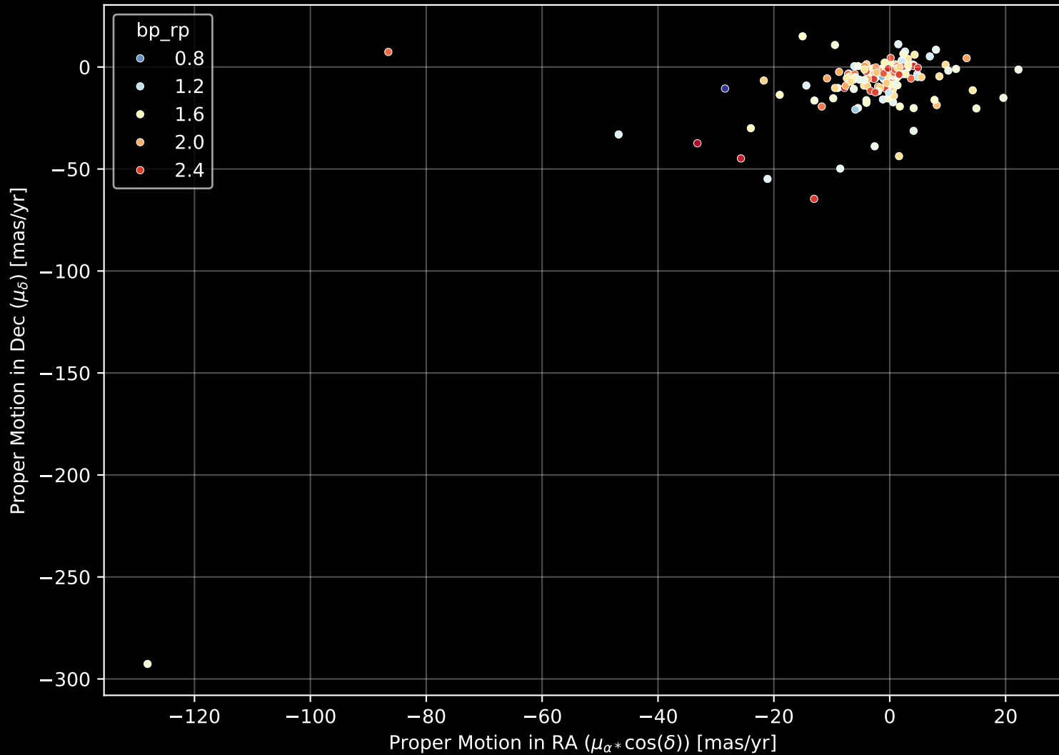
APOGEE DR17 Field: [K2_C11_003+05_btx] Proper Motion Diagram (n= 175)
