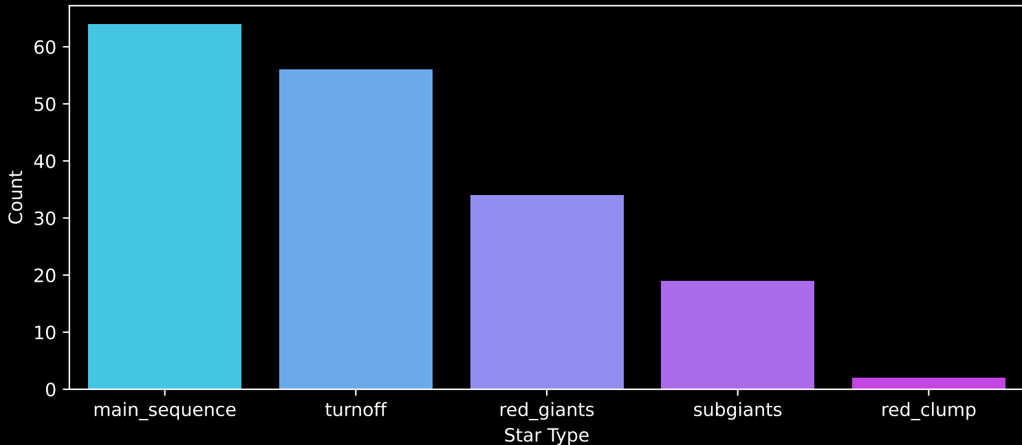
APOGEE DR17 Field: [K2_C11_003+05_btx] Count plot of Star Type
