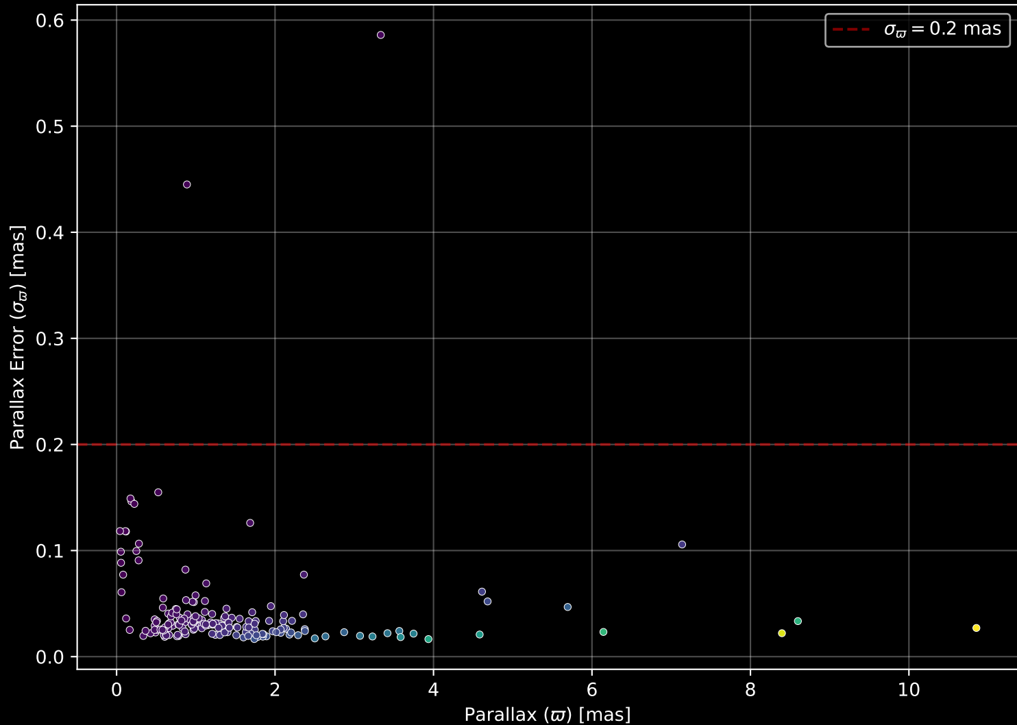
APOGEE DR17 Field: [K2_C11_003+05_btx] Parallax Quality (n= 175)
